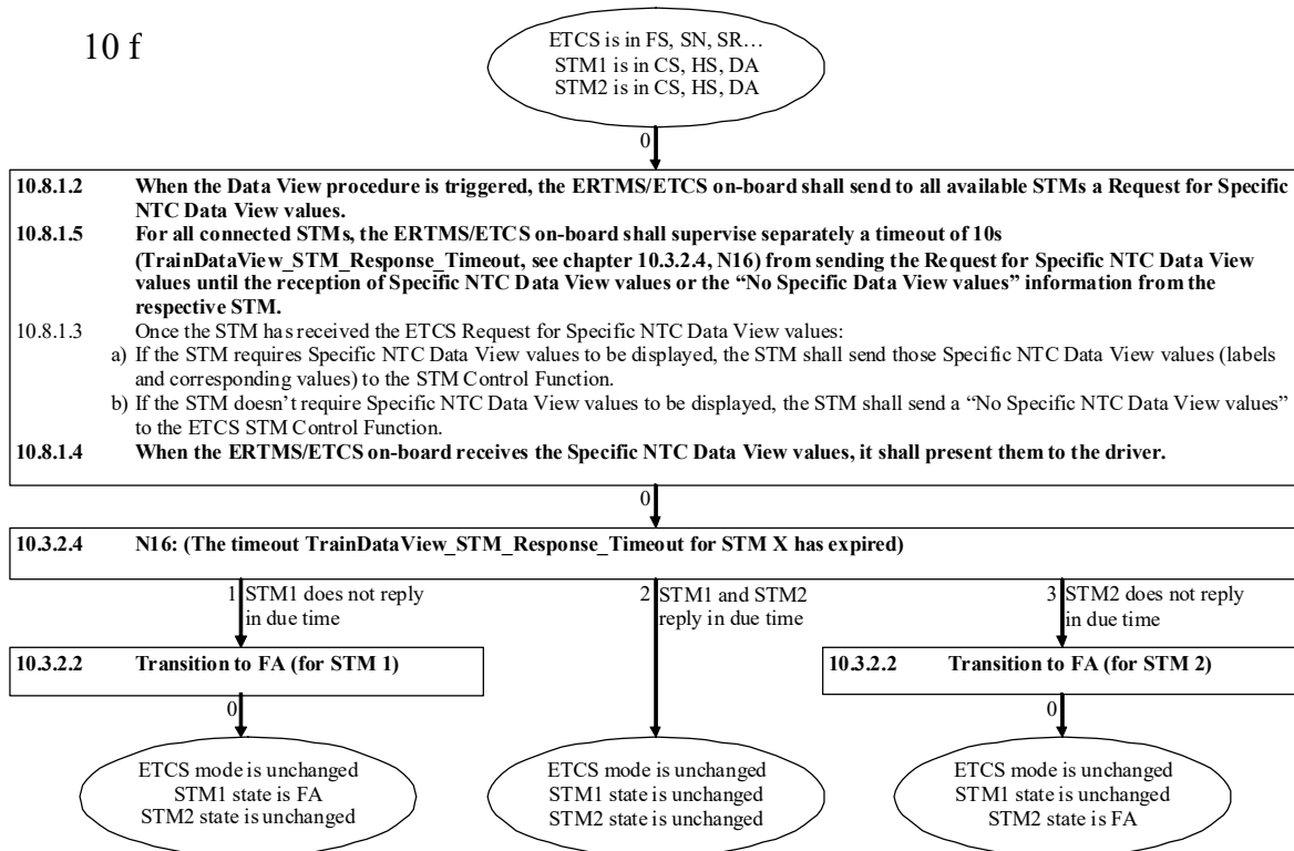
Figure 3: Test Diagram example
