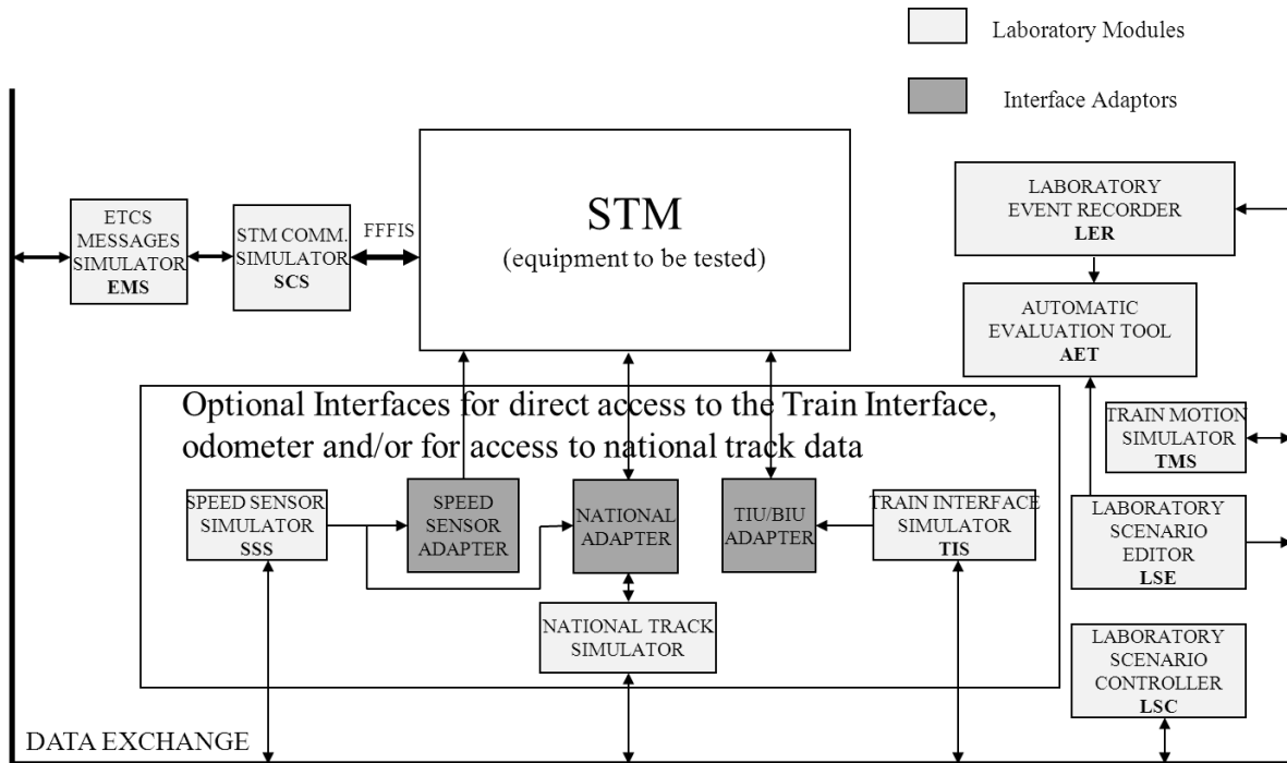
Figure 2: Test facility for the STM test
