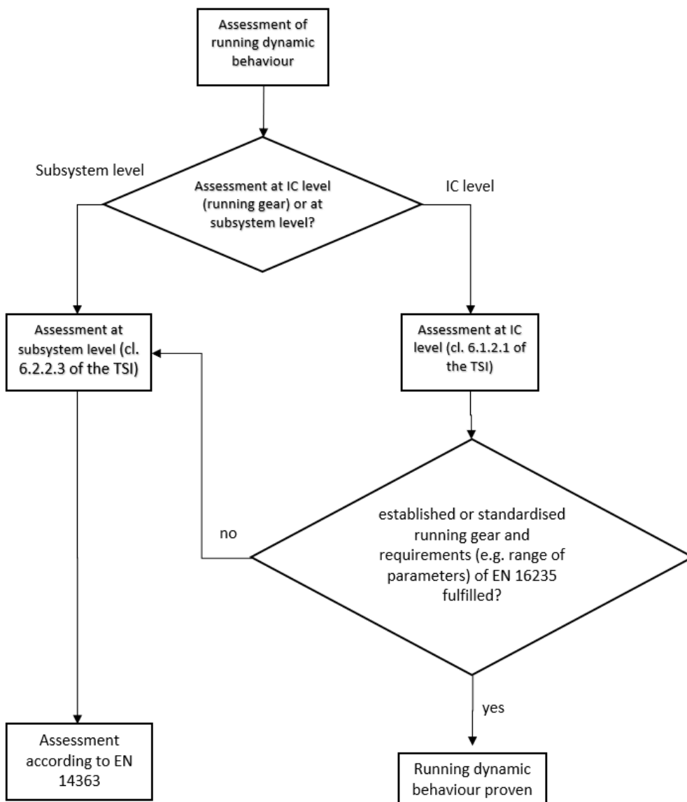
Figure 9: Flow chart of all the possibilities to prove the running dynamic behaviour in the TSI TSI perspective
