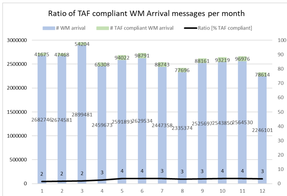
Diagram 8: Ratio of TAF compliant WM Arrival messages per month
