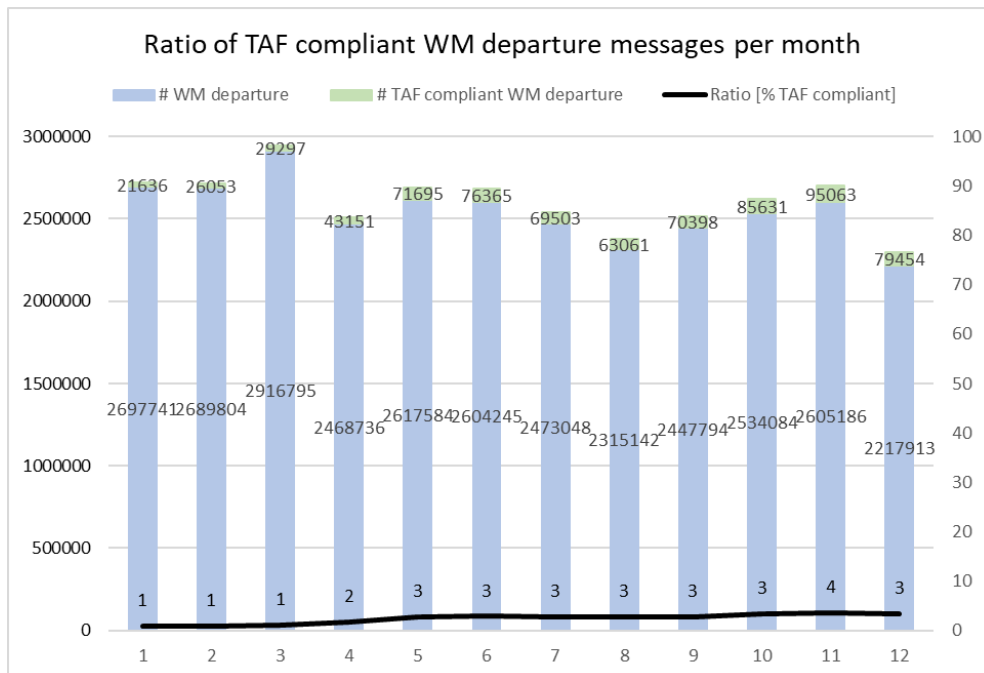
Diagram 7: Ratio of TAF compliant WM departure messages per month
